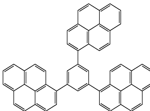
1,3,5-TPB
