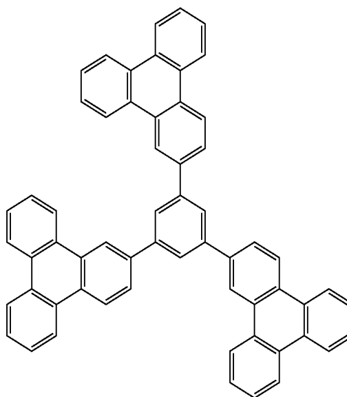
1,3,5-TTB
